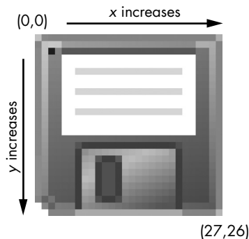
Figure 19-1: The x - and y -coordinates of a 28x27 image of some sort of ancient data storage device
