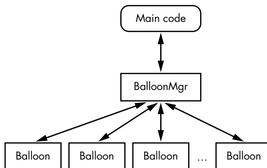
Figure 11-5: An object diagram of the Balloon game
